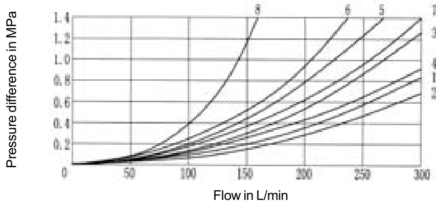
\Delta p/q_v -characteristic curves-Spool E
