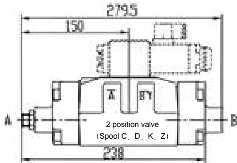
Stroke limiter on valve side A 11
