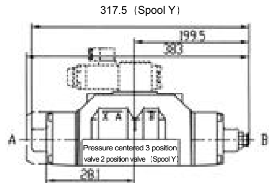
Stroke limiter on valve side B
