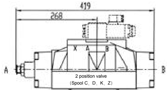
Stroke limiter on valve side A 11
