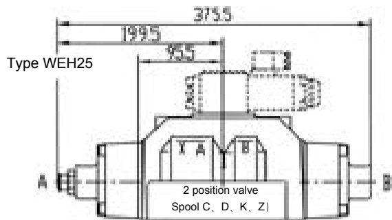
Stroke limiter on valve side A 11
