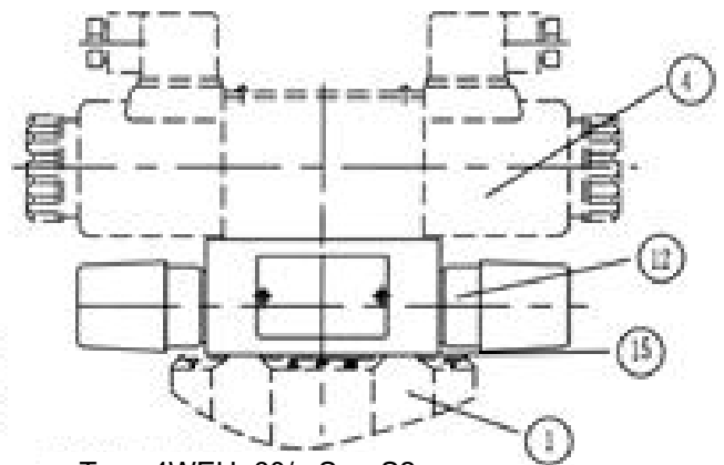
Type 4WEH..60/...S or S2
