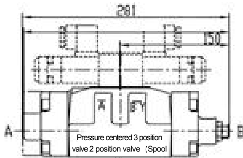
Stroke limiter on valve side B 12
