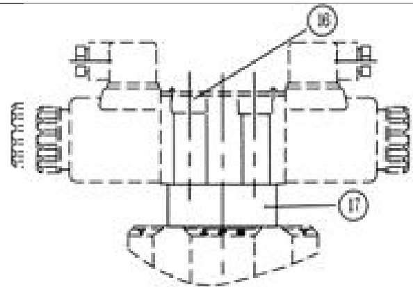
Type 4WEH..60/.../..D3
