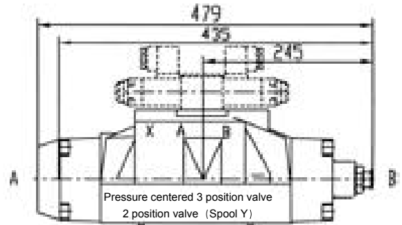
Stroke limiter on valve side B 12
