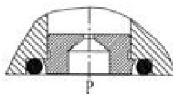
Cartridge throttle
