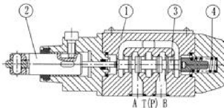
Type 4WMR6
