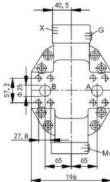
SAE flange ports A/B at rear, opposite(01)
