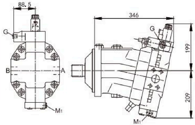
EP.D electric control, fixed setting
