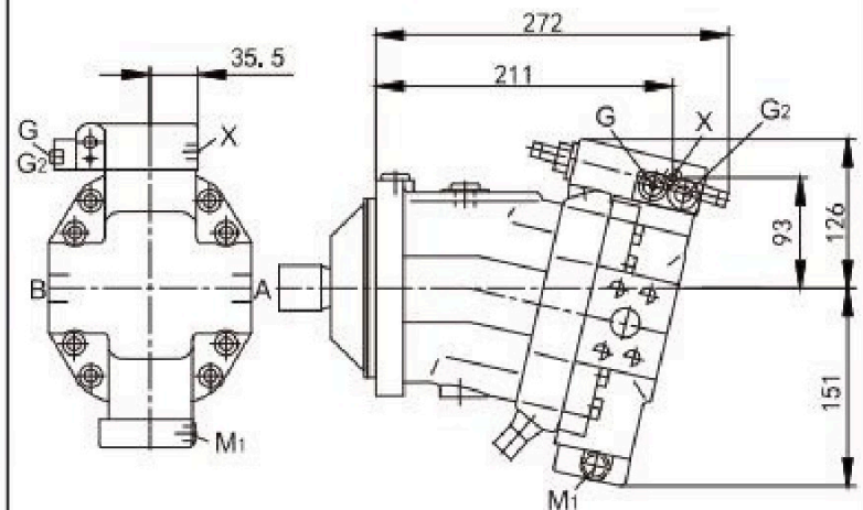
HD.E pressure control, two-point hydraulic override control
