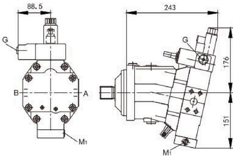
EP.D electric control, fixed setting
