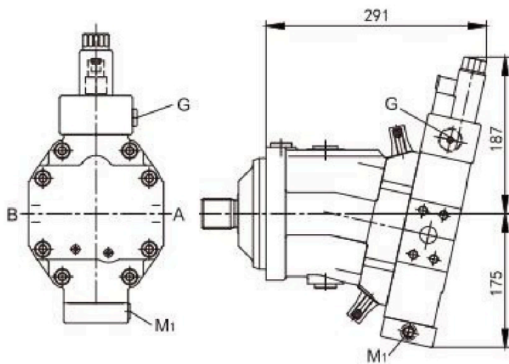
EP1/EP2 electric control, with proportional solenoid
