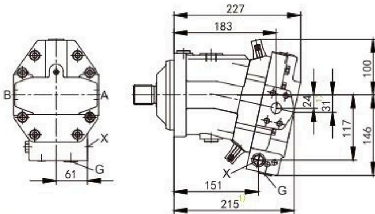
EZ3 two-point hydraulic control
