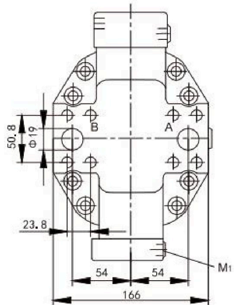
SAE flange ports A/B at rear, opposite(01)
