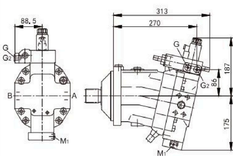
EP.E electric control, two-point hydraulic override control
