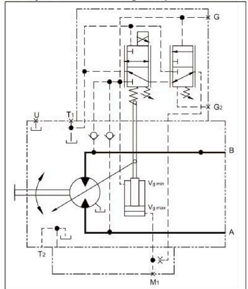
EP.E Hydraulic control circuit diagram-displacement 28-215
