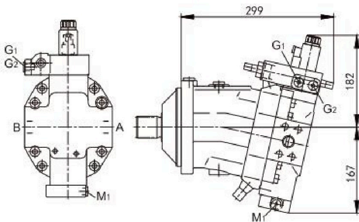
EP,E electric control, two-point hydraulic override control
