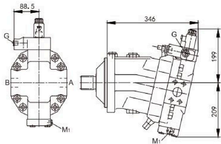
EZ.D electric control, two-point hydraulic override control
