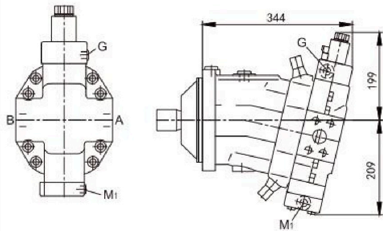
EZ1/EZ2 two-point electric control, with switching solenoid
