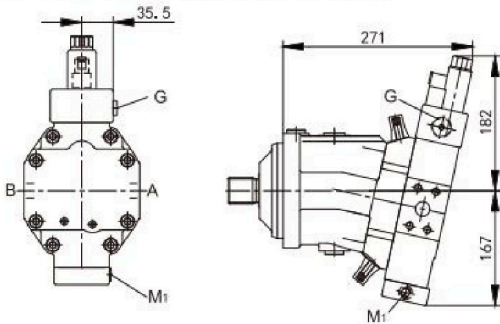
EP1/EP2 electric control, with proportional solenoid
