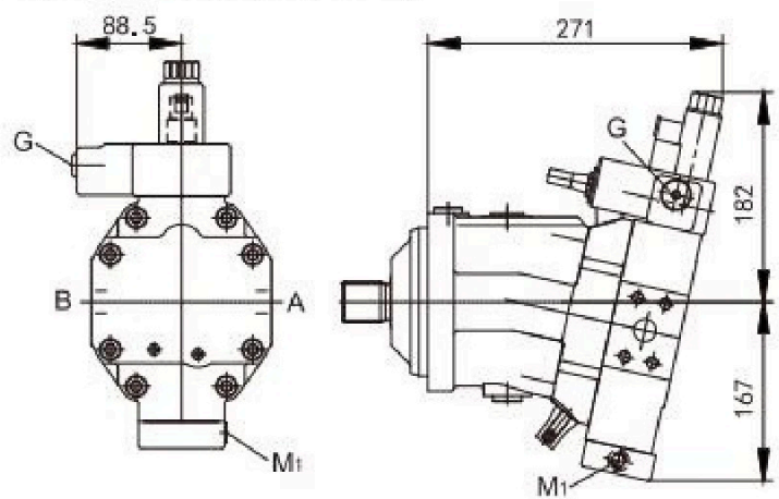
EP,D electric control, fixed setting
