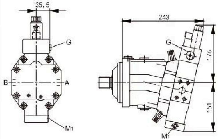
HP1/HP2 electric control, with proportional solenoid
