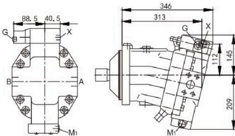
HD.D pressure control, fixed setting
