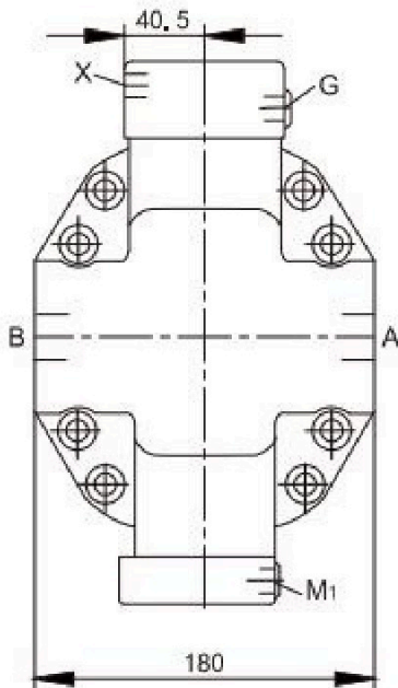
SAE flange ports A/B at side, opposite(02)
