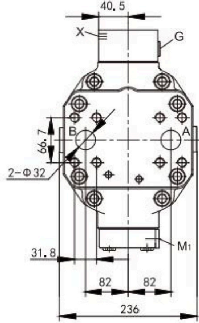
SAE flange ports A/B at rear, opposite(01)
