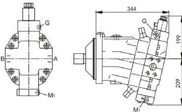
EZ3/EZ4 two-point electric control, with switching solenoid
