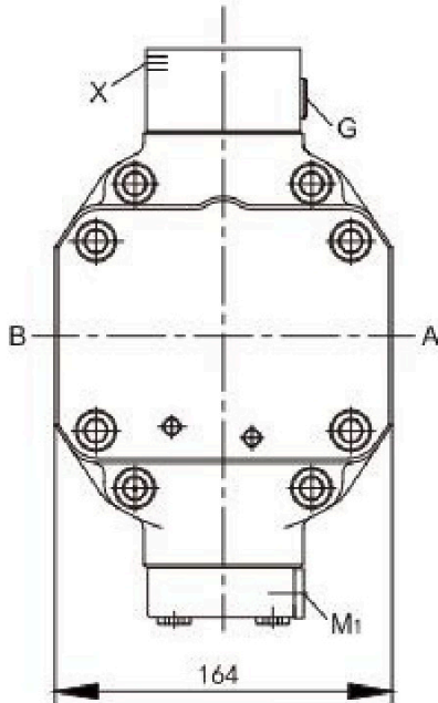
SAE flange ports A/B at side, opposite(02)
