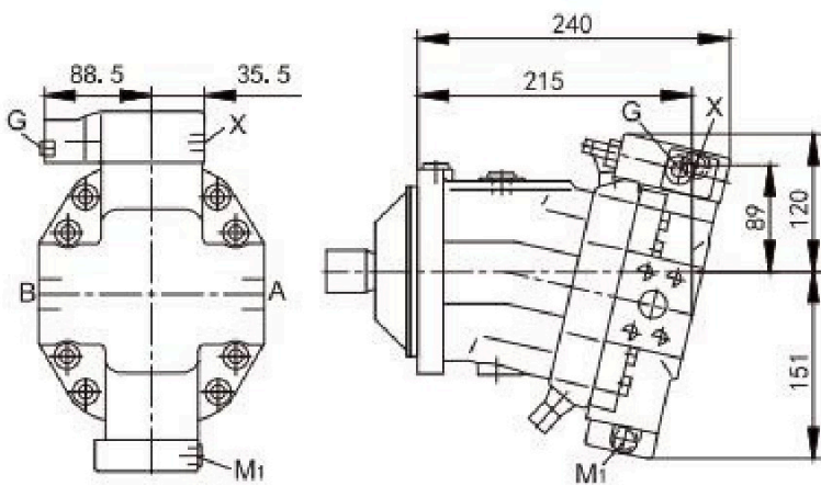
HD.D pressure control, fixed setting
