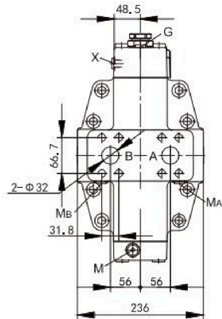
SAE flange ports A/B at rear, opposite(01)
