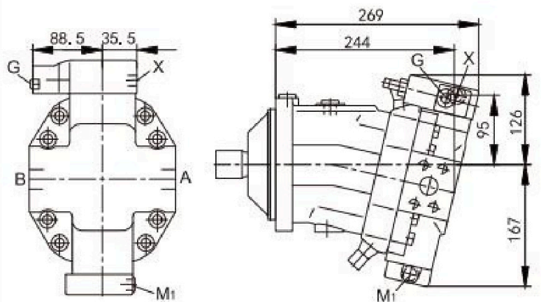
HD,D pressure control, fixed setting
