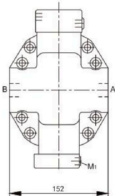
SAE flange ports A/B at side, opposite (02), only for HZ3/EZ3/EZ4
