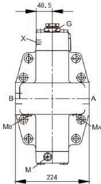
SAE flange ports A/B at side, opposite(02)
