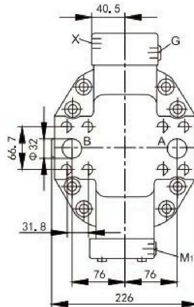
SAE flange ports A/B at rear, opposite(01)
