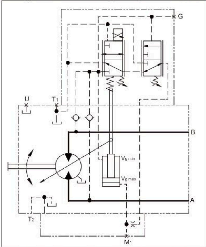
EP.D Hydraulic control circuit diagram-displacement 250
