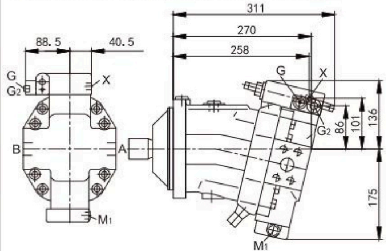
HD.E pressure control, two-point hydraulic override control
