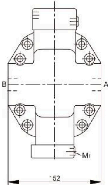
SAE flange ports A/B at side, opposite(02)
