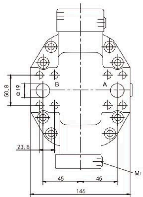
SAE flange ports A/B at rear, opposite(01)
