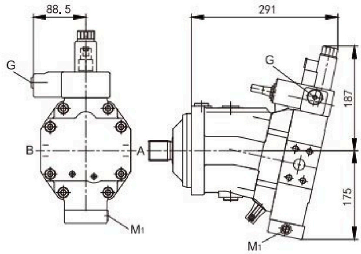
EP.D electric control, fixed setting
