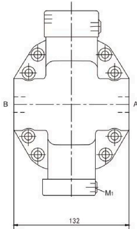
SAE flange ports A/B at side, opposite(02)
